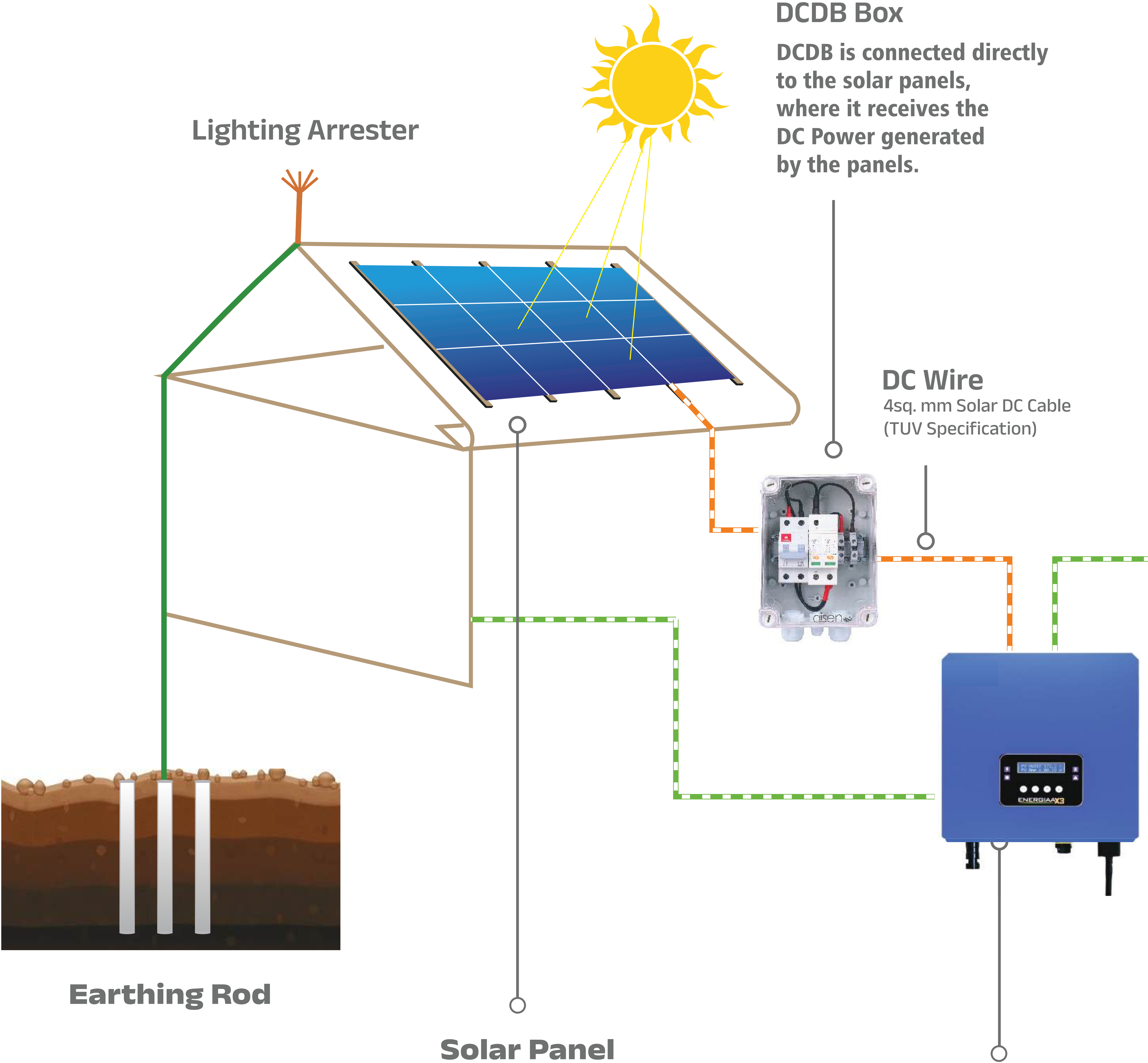
Solar Inverter
